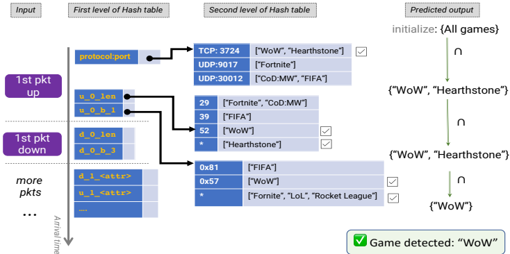
Fig. 1: The structure of our classifier, illustrating a progressive classification of a flow.
