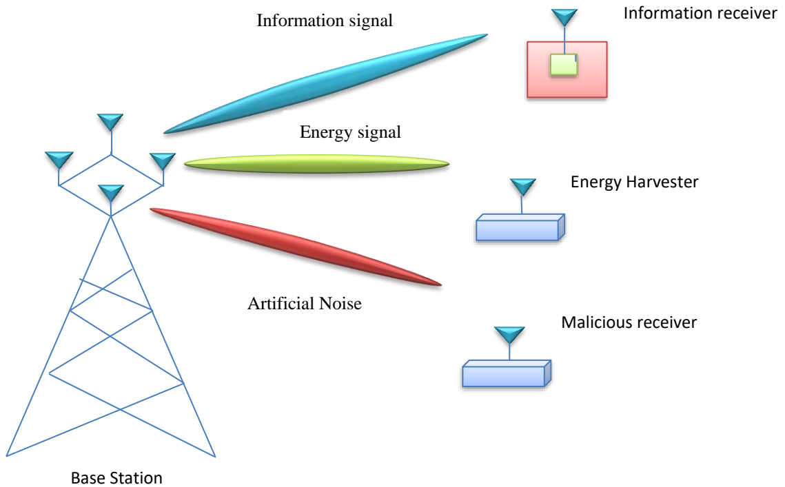
Figure 17: Beam forming in SWIPT system.
