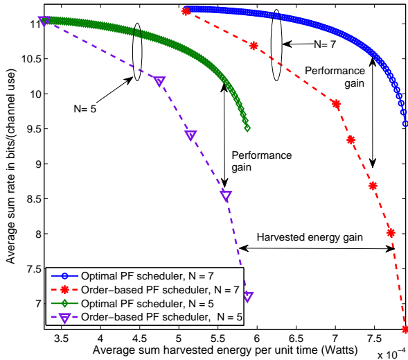
Fig. 3. Average sum rate versus average sum harvested energy of the PF schemes for different numbers of UTs.
