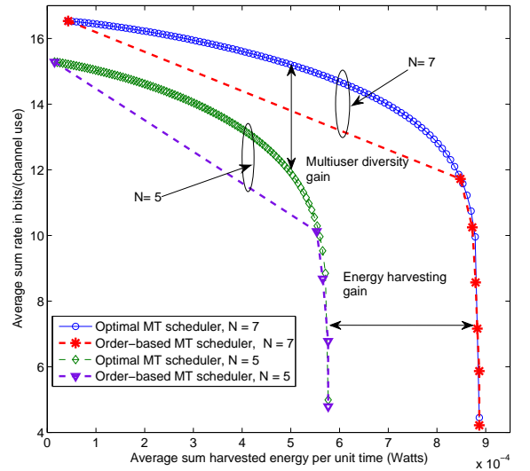
Fig. 2. Average sum rate versus average sum harvested energy of the MT schemes for different numbers of UTs.
