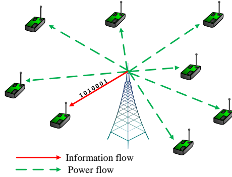
Fig. 1. A multiuser system with SWIPT for N = 8 time-switching user terminals (UTs).
