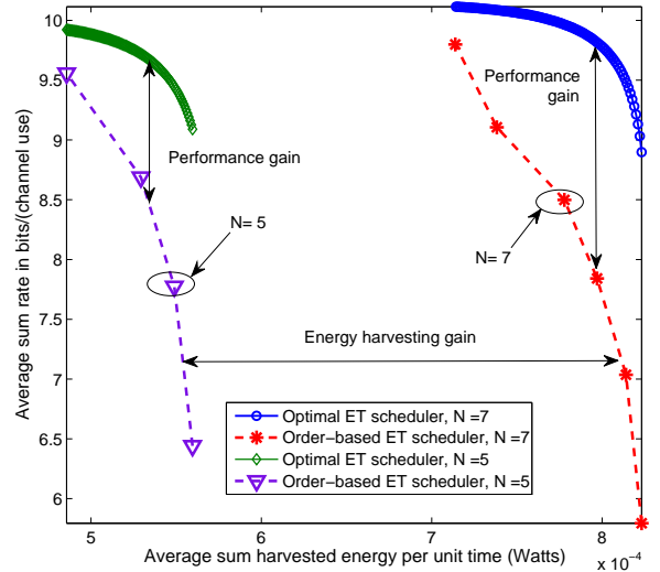
Fig. 4. Average sum rate versus average sum harvested energy of the ET schemes for different numbers of UTs.
