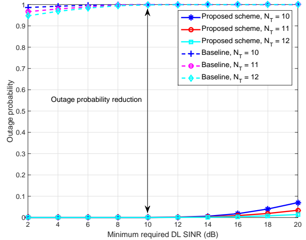
Fig. 4. Outage probability versus the minimum required DL SINR (dB), \Gamma_{req}^{DL} , for different resource allocation schemes.
