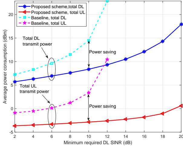
Fig. 3. Average power consumption (dBm) versus the minimum required DL SINR (dB), \Gamma_{req}^{DL} , for different resource allocation schemes.
