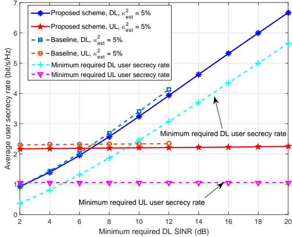
Fig. 6. Average user secrecy rate (bits/s/Hz) versus the minimum required DL SINR (dB), \Gamma_{\text{req}}^{\text{DL}} .
