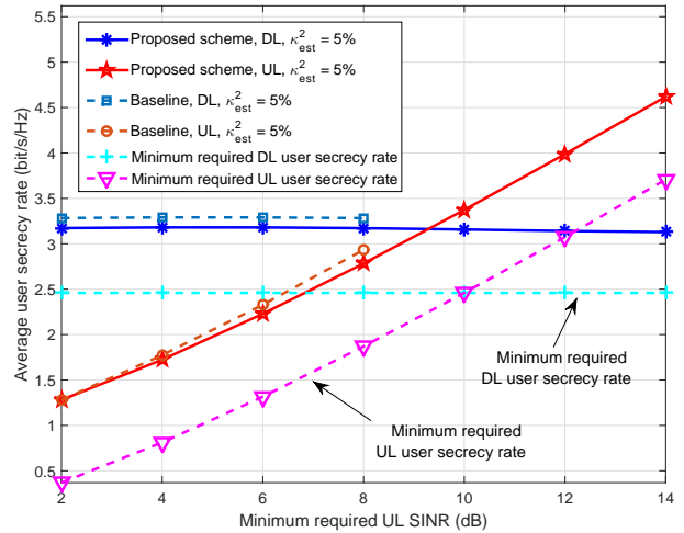
Fig. 7. Average user secrecy rate (bits/s/Hz) versus the minimum required UL SINR (dB), \Gamma_{\text{req}}^{\text{UL}} .
