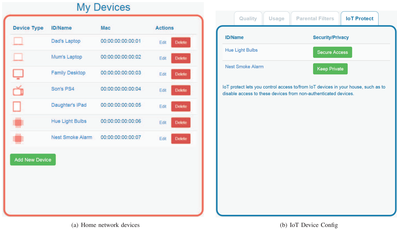
Fig. 3. Web interface showing (a) devices, (b) bandwidth, (c) filters, and (d) usage.
