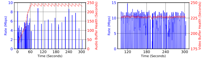
(a) Audio buffer (on client) versus corresponding flow (on network). (b) Video buffer (on client) and corresponding flow (on network).
