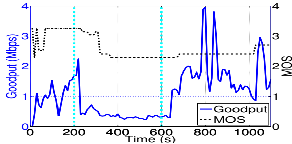
Fig. 11. YouTube streaming.
