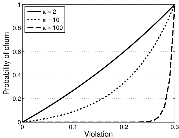
Fig. 2. Churn probability.
