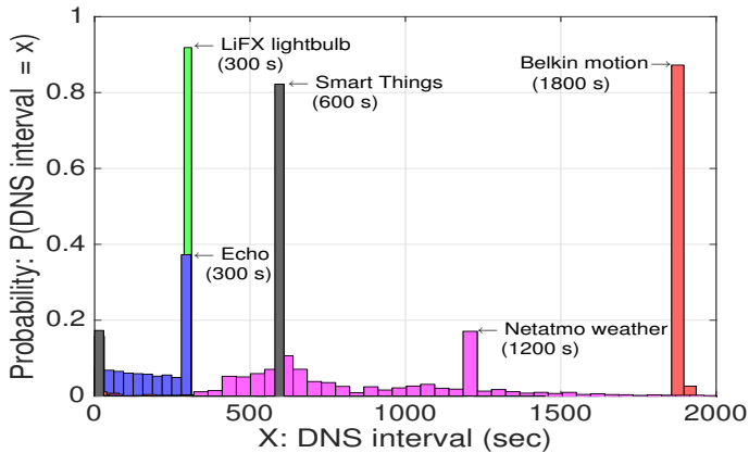
Fig. 6. Histogram of DNS interval.
