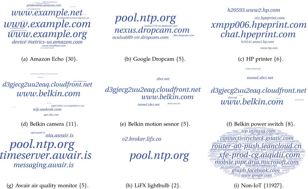
Fig. 5. Word-cloud of domain names (total count of unique domains is shown in {sub-captions} next to the device name).
